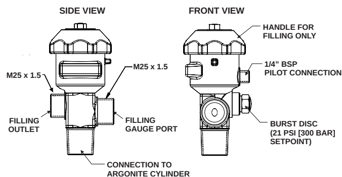
Figure 4. Argonite Cylinder Valve
