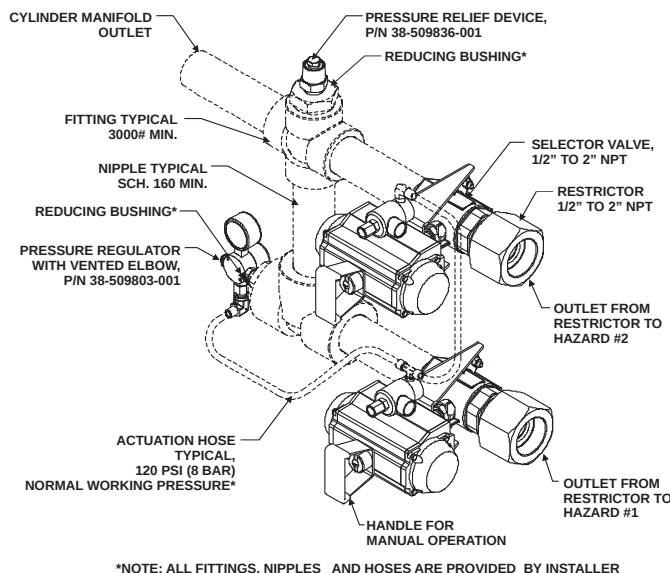
Figure 14. Selector Valve System
