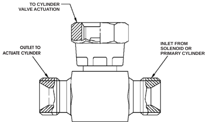
Figure 8. Tee Piece
