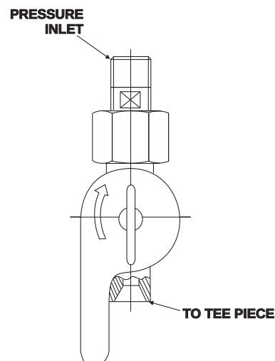
Figure 7. Manual/Pneumatic Actuator
