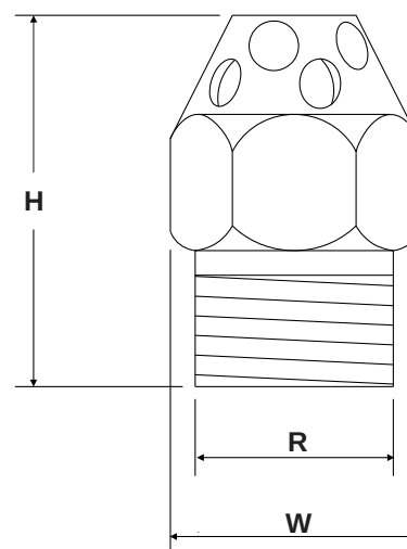
Figure 15. Nozzles (37 mm)
